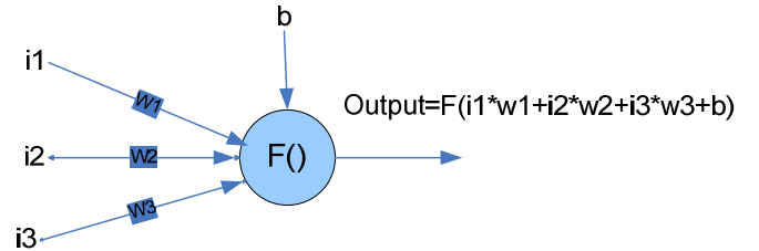
Fig 13. A single processing element in ANNs
