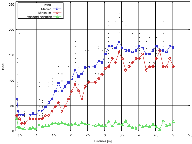
Fig 11. RSSI measures using 10cm step size
