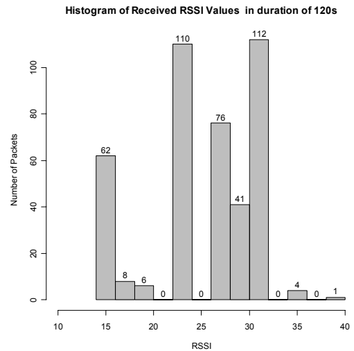
Fig 2. Variation of the RSSI values over 120s
