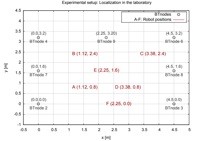
Fig 2. Experimental setup for localization including anchor nodes (BTnode2 ... BTnode9) and searched positions (A ... F)
