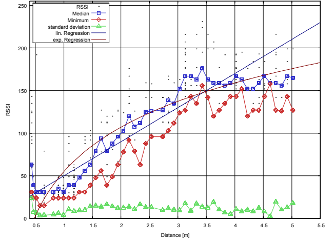
Fig 12. Linear and exponential regression based on the median of the measured RSSI values
