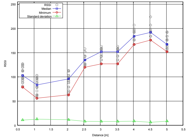
Fig 9. RSSI values measured at 869.9 MHz
