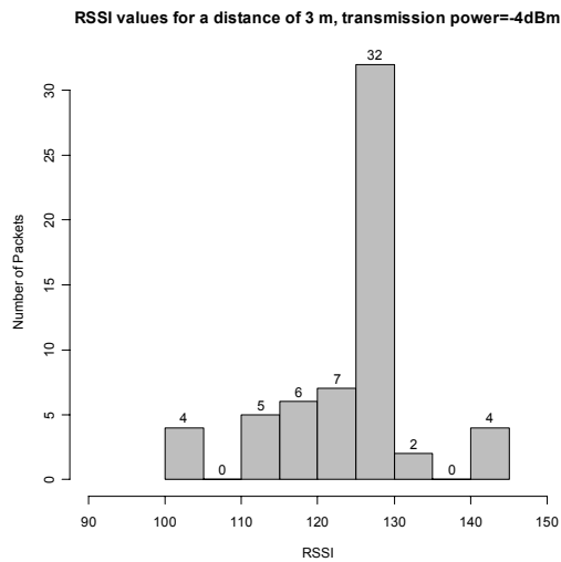
Fig 7. RSSI measurement for 3m, transmission power -4 dBm
