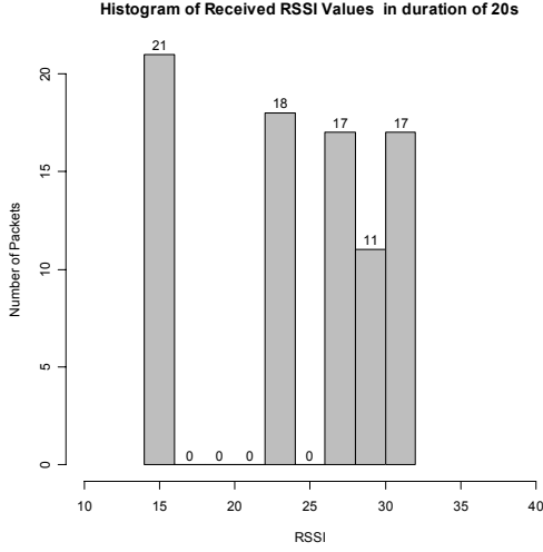
Fig 3. Variation of the RSSI values over 20s
