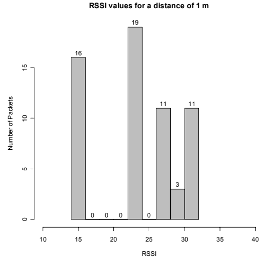
Fig 4. RSSI measurement for 1m
