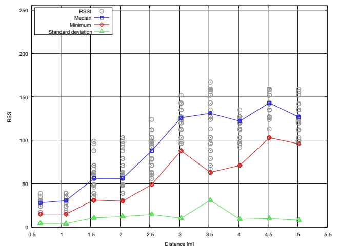
Fig 10. RSSI values measured during rotation
