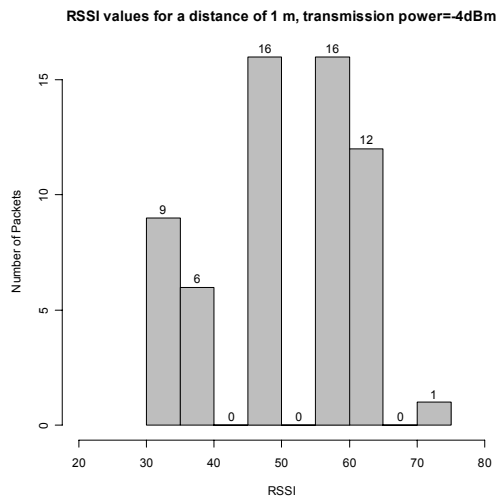
Fig 6. RSSI measurement for 1m, transmission power -4 dBm
