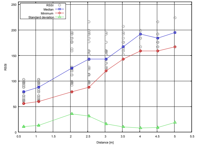
Fig 8. RSSI values measured at 863.5 MHz
