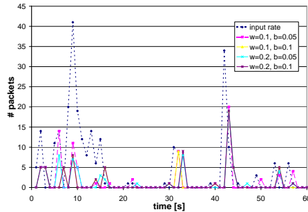
Fig. 10. Output rate for variable detection ratio and fixed timeout (10s)
