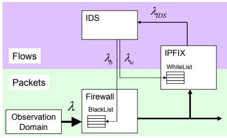
Fig. 3. Basic model for adaptive re-configuration including the main components and the control and data flows
