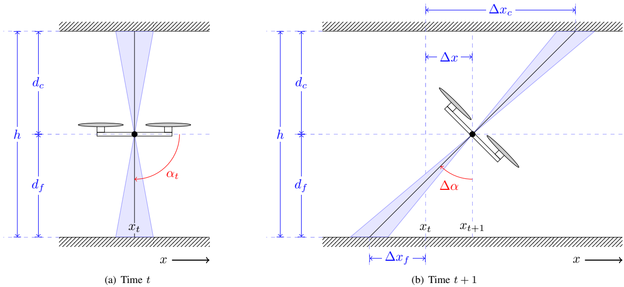
Fig. 5. Quadrotor movement
