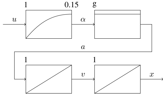
Fig. 4. System model of a copter
