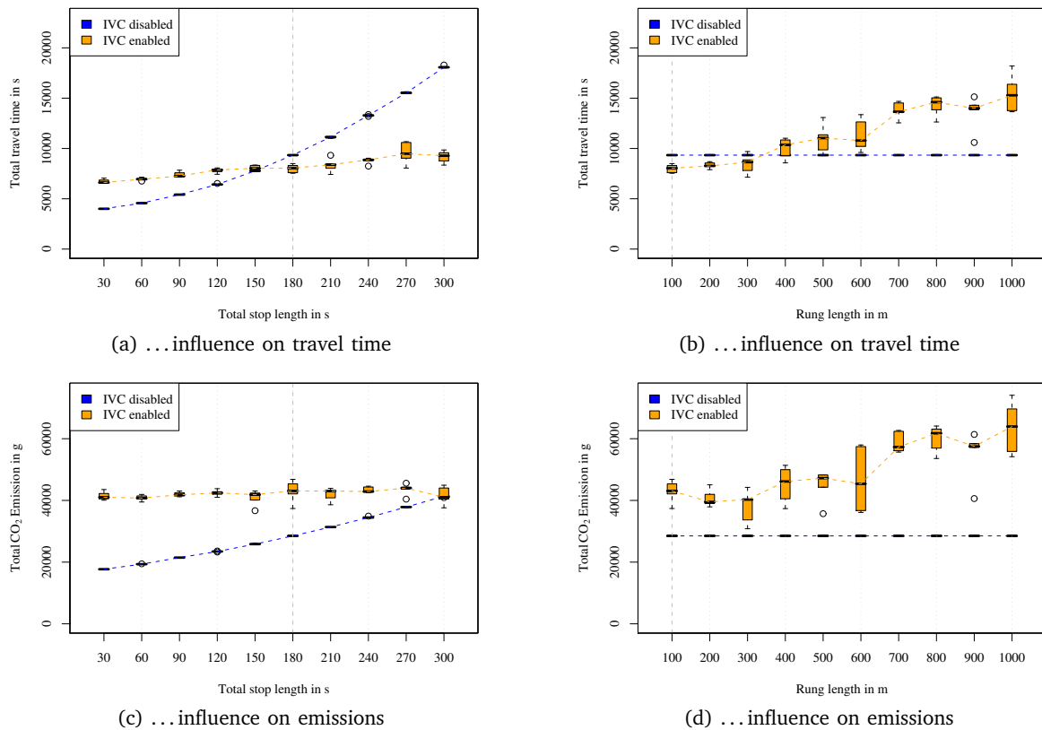
Figure 5. Influence of stop time and rung length on travel time and CO 2 emissions; multiple stops
