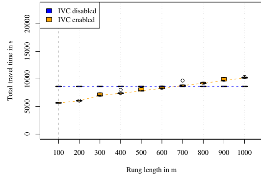
(b) ... influence on travel time
