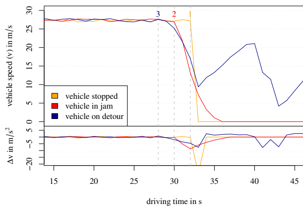
Figure 3. Impact of route choice on vehicle speed and acceleration profile
