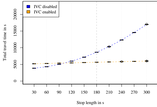
(a) ... influence on travel time
