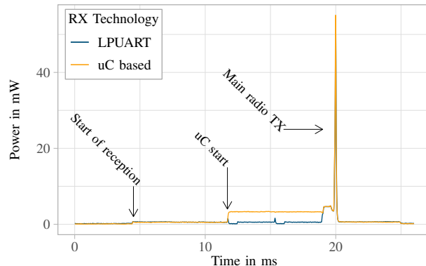
Fig. 6. Power consumption of prototype (with & without the LPUART) during reception of LPD frame and subsequent uplink transmission of a packet over the main radio.
