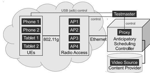
Figure 6. Testbed Architecture
