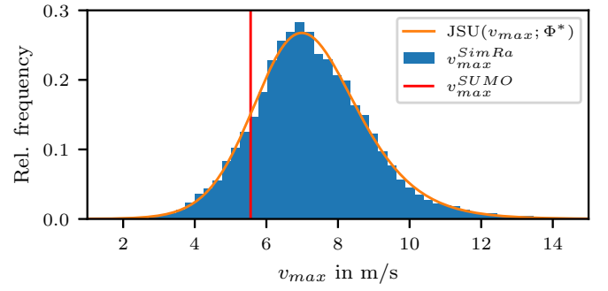
Figure 2. Histogram of the empirical maximum velocity data and the fitted JSU. The red scalar represents the default value in SUMO.
