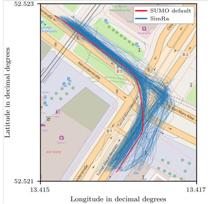
Figure 3. Qualitative comparison between the SUMO default intersection model and real world data given by SimRa for the intersection between Alexanderstraße and Karl-Marx-Allee in Berlin. SimRa shows two distinct left-turn paths (i.e., a direct and an indirect one) whereas SUMO default only models the direct path.
