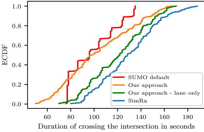
Figure 9. ECDFs of the measured durations for crossing the scenario Mehringdamm . The results when using our new approach are only slightly more realistic than when using the standard SUMO model. However, when the direct path is blocked for cyclists, the simulation results outperform the default approach.
