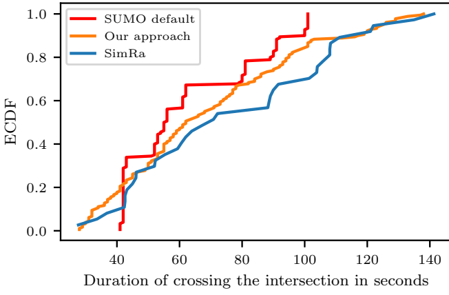
Figure 8. ECDFs of the measured durations for crossing the scenario Warschauer Straße . It is apparent that our approach outperforms SUMO’s default as the measured durations converge towards the real-world data.
