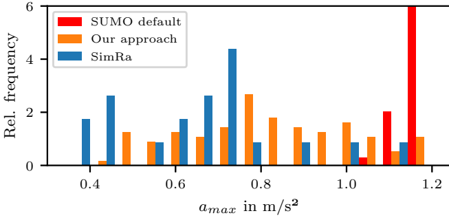
Figure 5. Histogram of SUMO's, SimRa's, and our approach's observed maximum accelerations inside the example Oranienstraße scenario. While the maximum accelerations are heterogeneously distributed in the real-world data and our approach, the default values are clustered. Here, the observed accelerations deviate from the configured default value ( 1.2\text{m/s}^2 ) due to traffic effects inside the simulation.
