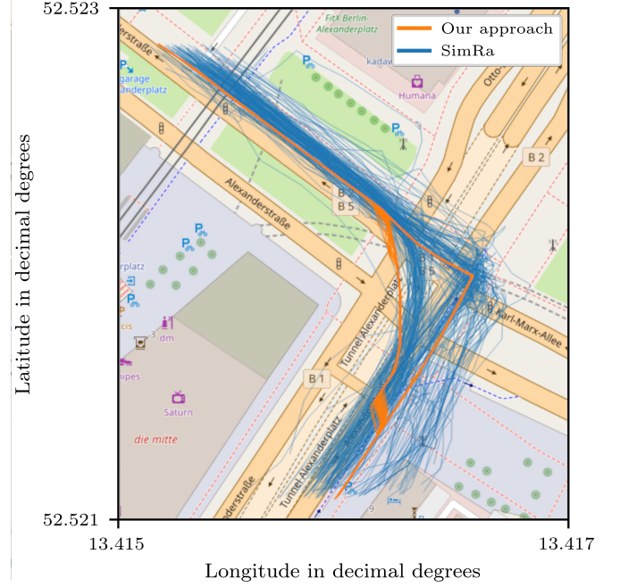
Figure 7. Qualitative comparison between the results of our approach for the intersection model and real-world data given by SimRa for the intersection between Alexanderstraße and Karl-Marx-Allee in Berlin. SimRa shows two distinct left-turn paths (i.e., a direct and an indirect one), which are also modeled by our approach.
