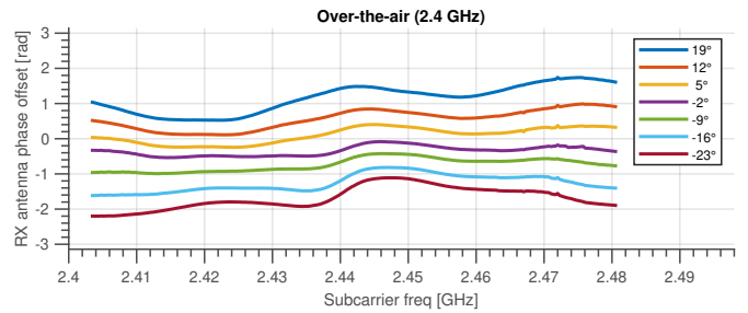
Figure 10. Estimated phase offset between the two receive antennas for the six different AoA values.
